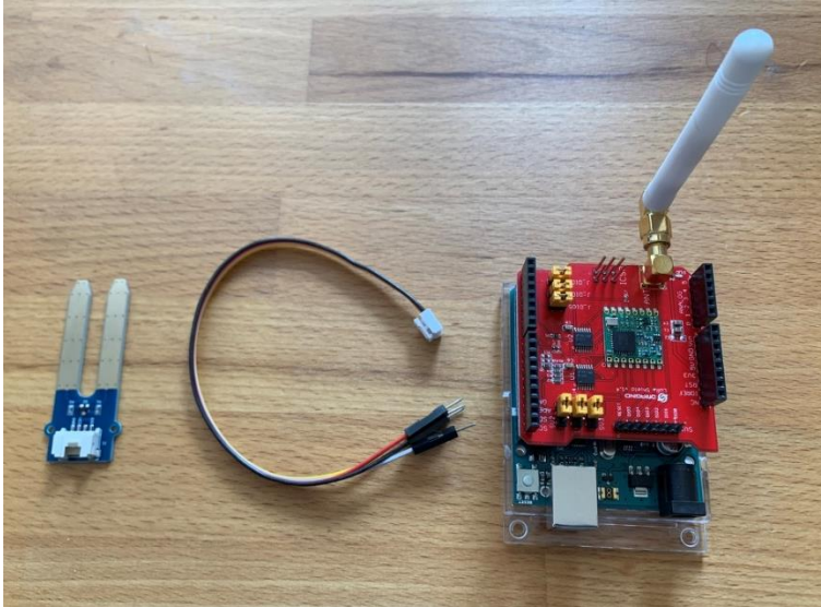
Figure 8: (left to right) Grove Moisture Sensor, JST to male jumper cable, assembled Arduino and shield
