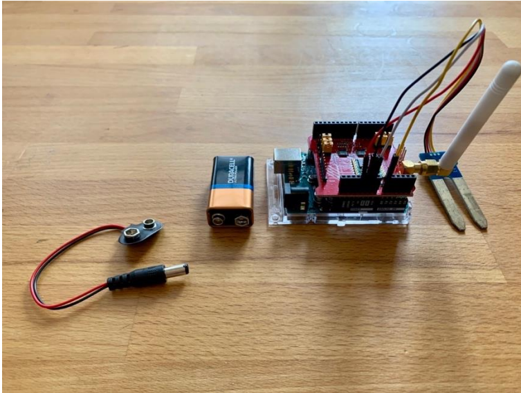
Figure 24: Left to right, battery clip, 9-volt battery, broadcasting node
