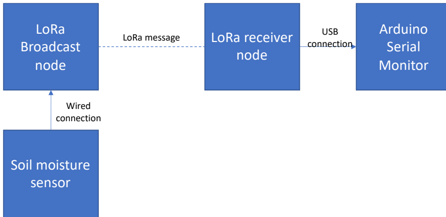
Figure 2: Schematic of the system for stages 1 and 2.
