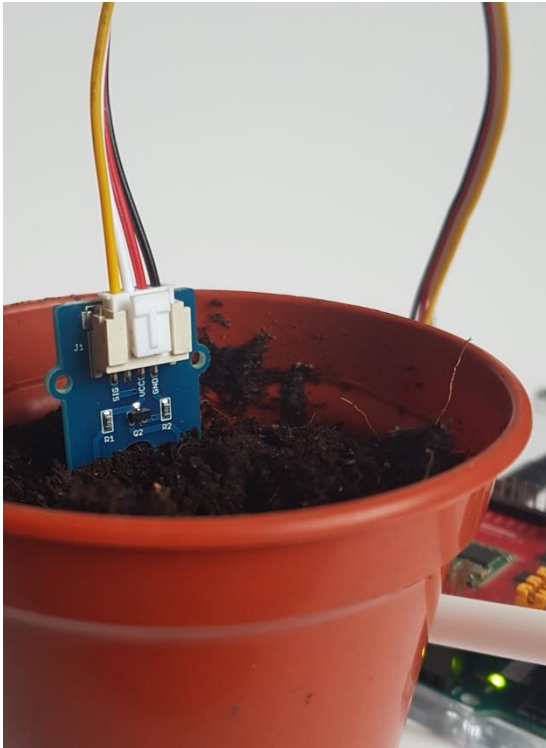
Figure 22: Testing the assembled moisture sensor
