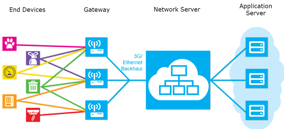
Figure 1: LoRaWAN network high level architecture.
