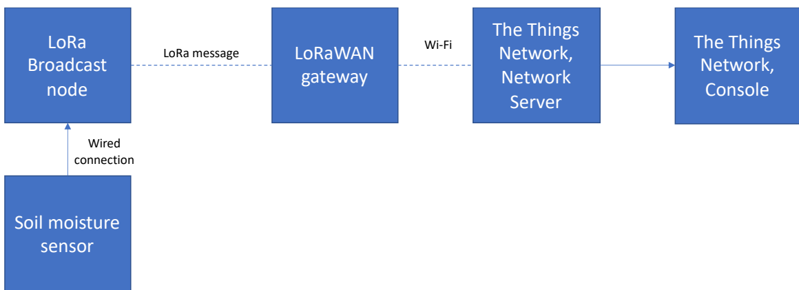
Figure 3: Schematic of the system for stage 3.
